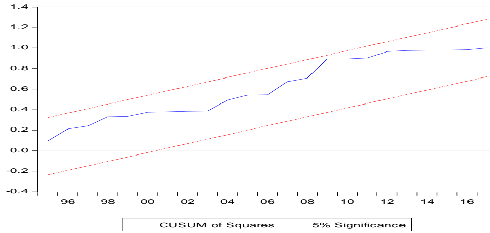
Figure 12A: Plot of CUSUMQ (United Arab Emirates)
