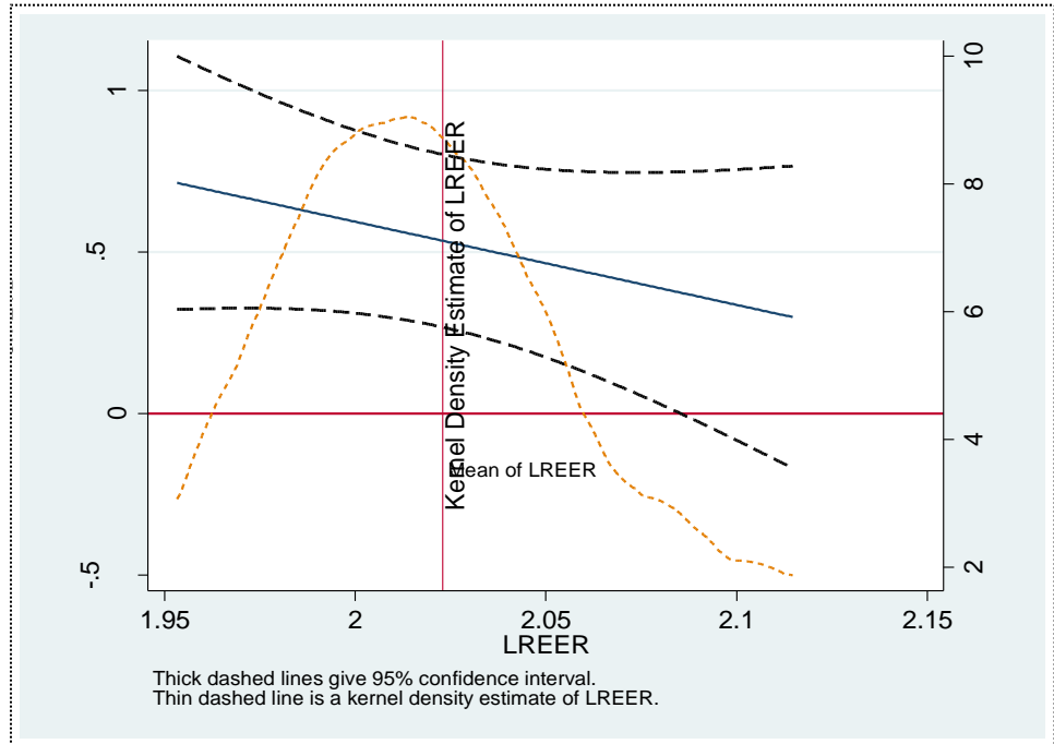
Figure 2: Marginal Effect Graph (Kuwait)
